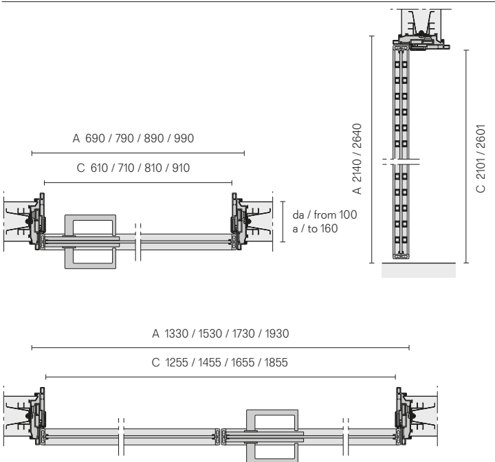
A. Luce netta falso telaio Measure of the subframe C. Luce netta passaggio Dimensions of the opening
