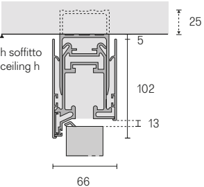
Monorotaia a soffitto Single ceiling rail
