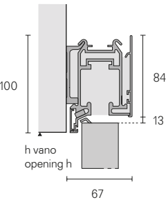
Monorotaia a parete Single wall rail
