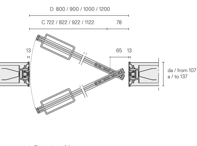
C. Luce passaggio Dimensions of the passage D. Luce vano Dimensions of the opening
