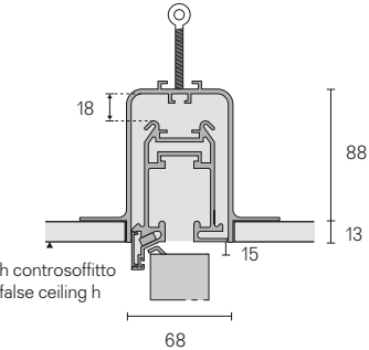
Monorotaia a incasso Single built-in rail
