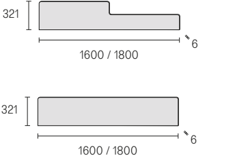
Alzatina in vetro con e senza sagomatura Glass upstand with and without shaping
