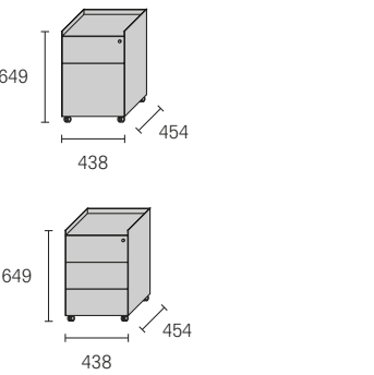
Porta documenti in metallo laccato Document holder in painted metal
