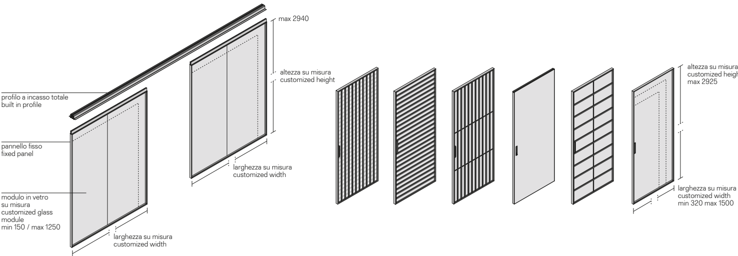
Porte abbinate al sistema interparete Spazio Doors combined with Spazio partition wall system
