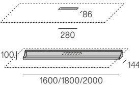
Passacavi in vetro e canalina raccogli cavi in alluminio Glass cable cut and aluminum cable ties
